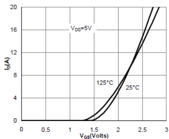
Transfer Characteristic
