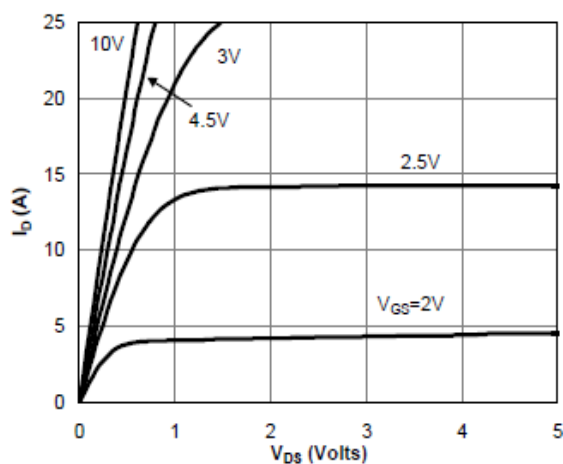
Output Characteristic
