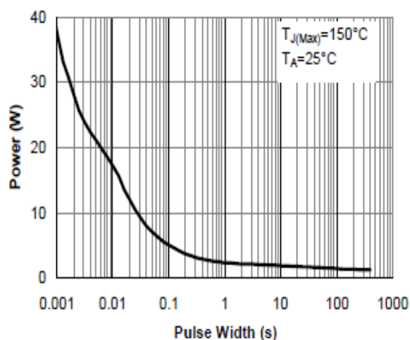
Figure 10: Single Pulse Power Rating Junction-to-Ambient (Note E)
