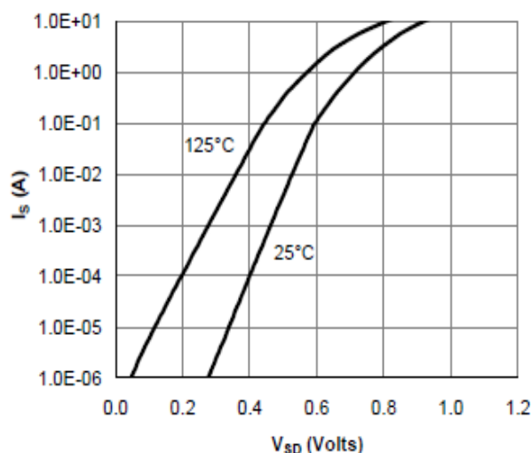
Body-Diode Characteristics
