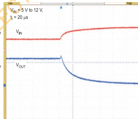
OVP RESPONSE FOR INPUT STEP
