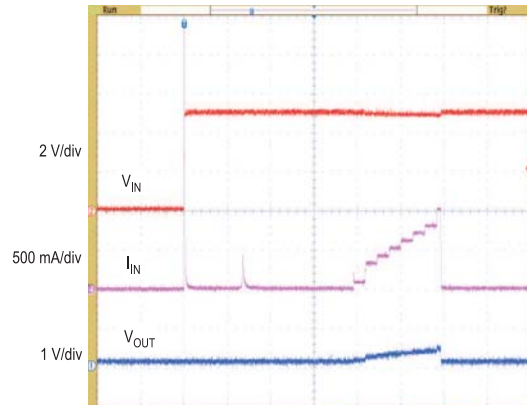
OCP, ZOOM-IN ON THE FIRST CYCLE OF FIGURE 7
