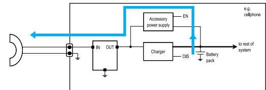
Figure 14 . Powering an Accessory - The Red Arrows Show the Direction of Current Flow
