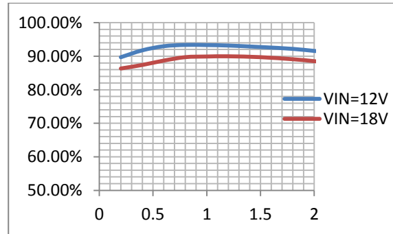
Efficiency @ V_{out}=5V
