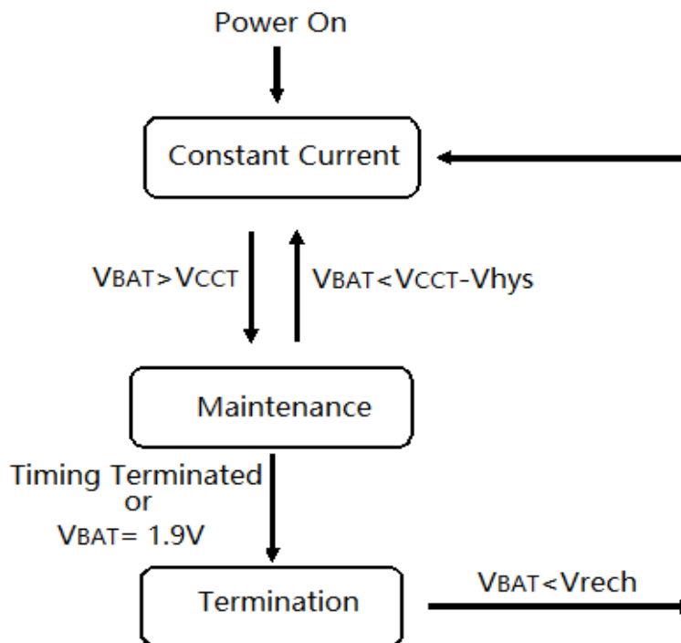
Figure 3 Charging Flow
