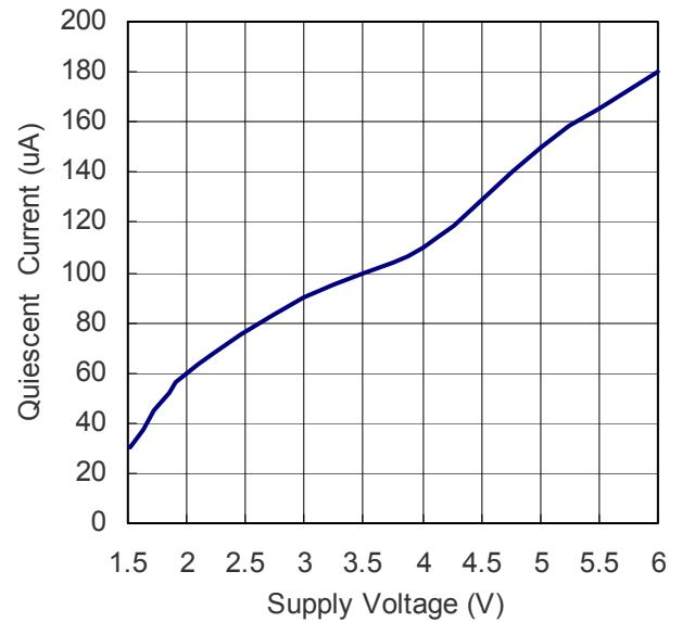
Quiescent Current vs. Supply Voltage (I o =0A)
