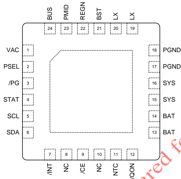
(QFN4x4-24)
