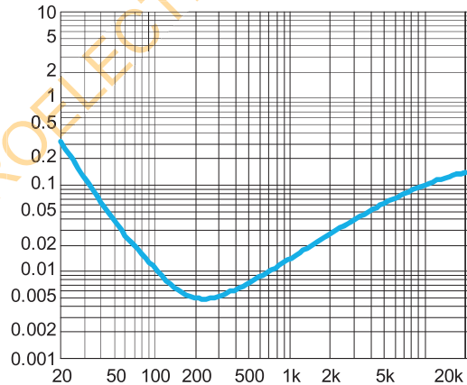
THD+N vs. Frequency SE mode, 3V, 320hm, P_o=20\text{mW}
