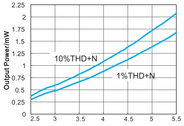
Output Power vs. Power Supply BTL mode, f=1 kHz, RL=8 Ohm
