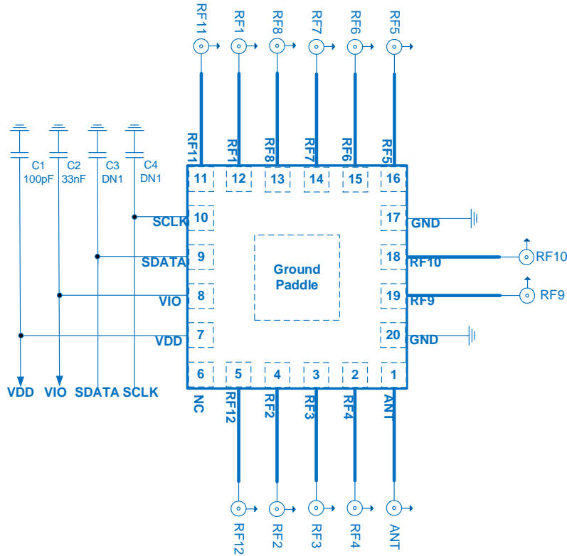
Figure 2 Evaluation Board Schematic
