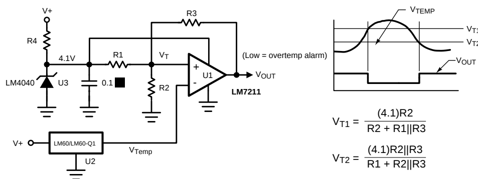
Figure 17. Centigrade Thermostat
