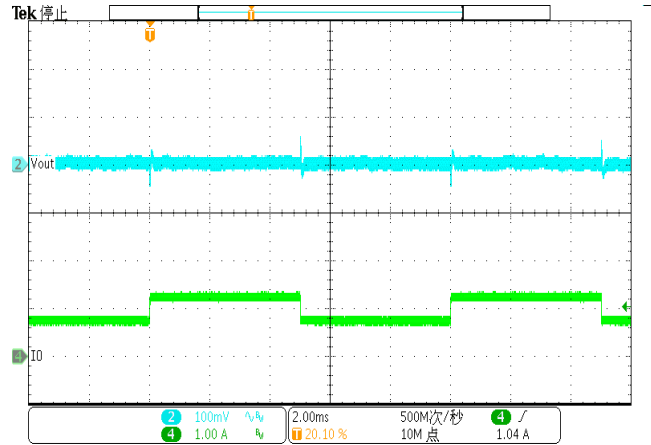
Figure 18. Load Transient (0.75A-1.25A, 1.6A/us)
