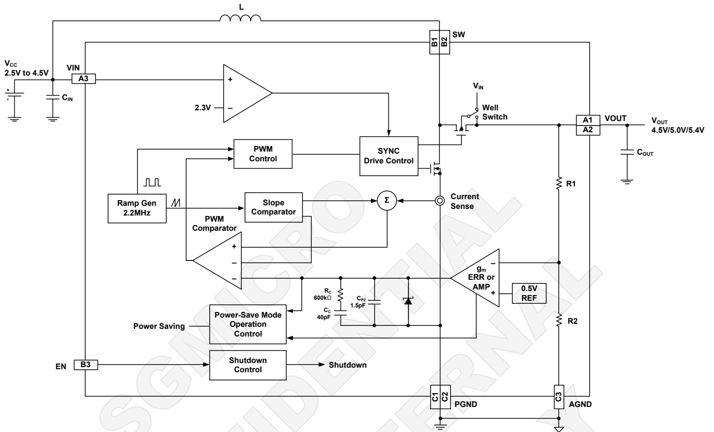
Figure 2. SGM66055 Block Diagram
