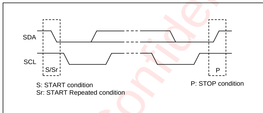
Figure 9 I²C Start/Stop Condition Timing
