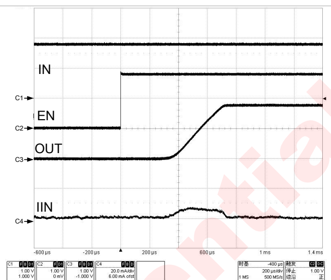
Figure 19 Inrush Current with C_{OUT}=1\mu F
