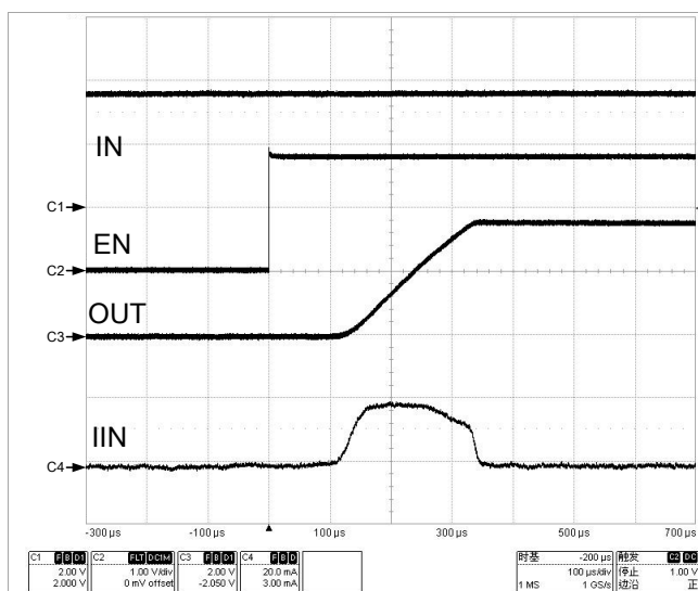
Figure 18 Inrush Current with C_{OUT}=1\mu F
