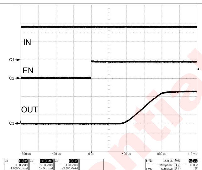
Figure 13 Turn On Response
