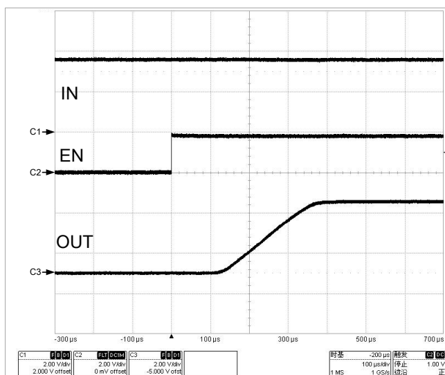
Figure 12 Turn On Response
