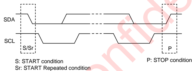
Fig 27 Start and Stop Conditions
