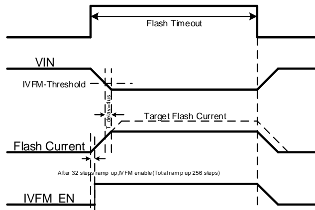
Fig 25 IVFM Timing
