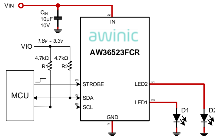
Fig 3 AW36523 Application Circuit
