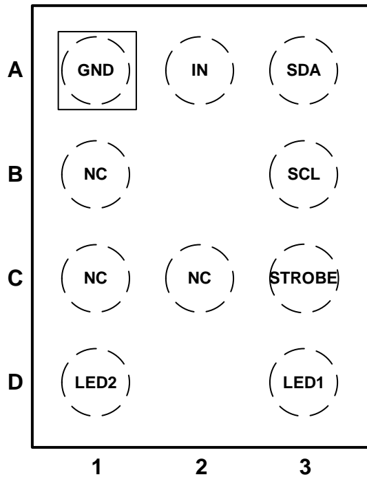
AW36523FCR Pin Configuration (Top View)
