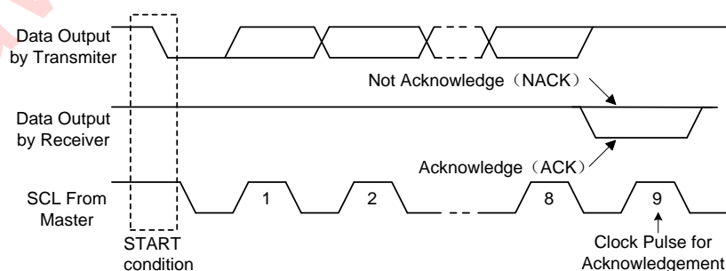
Fig 28 Acknowledgement Diagram
