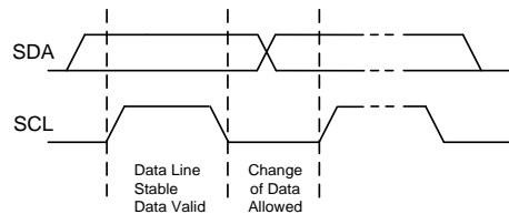
Fig 26 Data Validation Diagram
