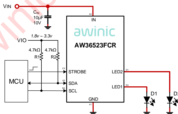
Fig 1 Typical Application Circuit of AW36523
