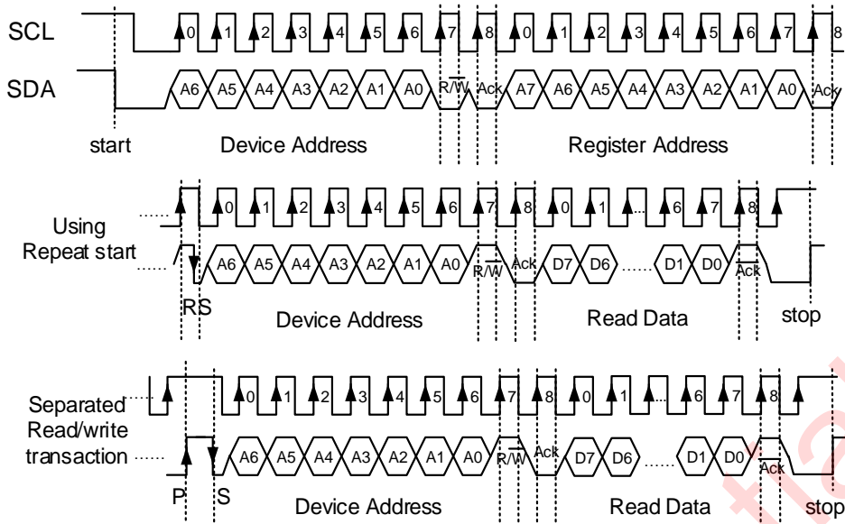
Fig 30 I 2 C Read Timing
