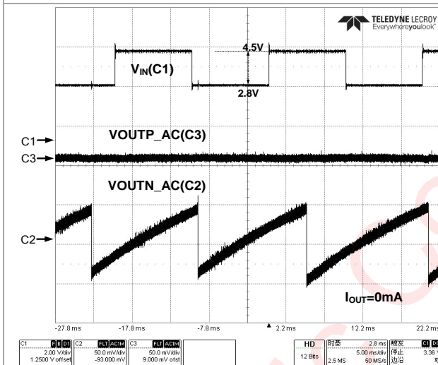
Figure 61 Line Transient (100mA Mode)
