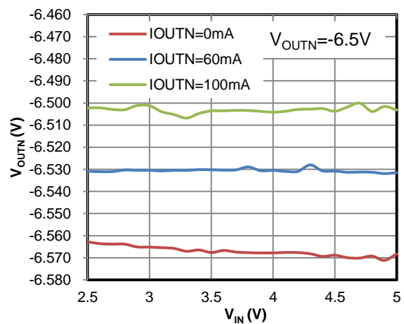
Figure 28 Line Regulation (100mA Mode)
