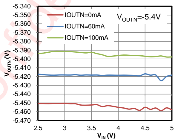
Figure 26 Line Regulation (100mA Mode)
