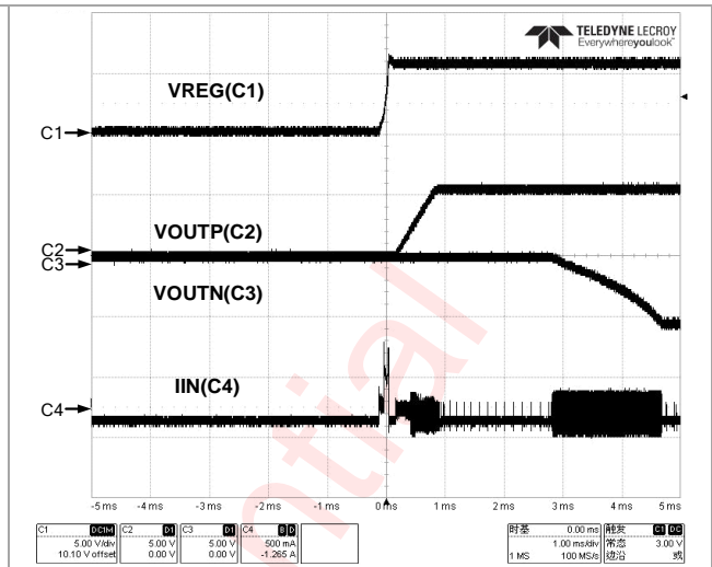
Figure 66 Inrush Current (Sequential)
