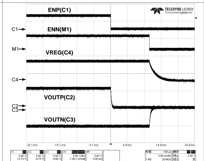
Figure 70 Power Down Sequencing (Sequential)
