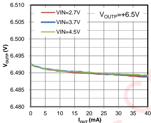
Figure 31 Load Regulation (40mA Mode)
