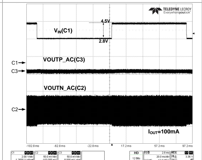
Figure 64 Line Transient (100mA Mode)
