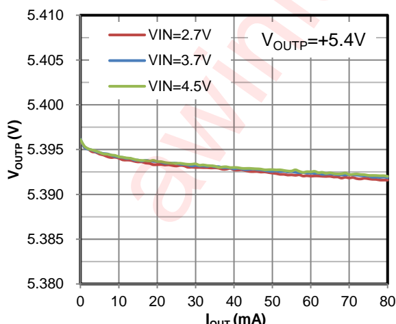
Figure 33 Load Regulation (80mA Mode)
