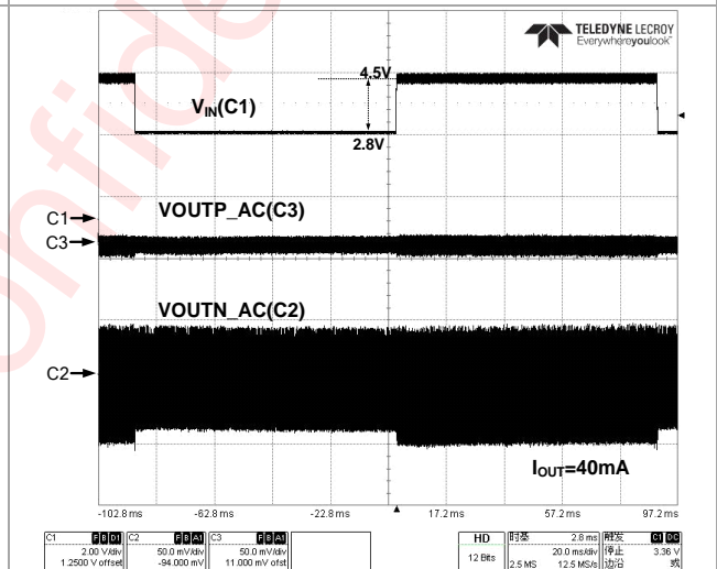
Figure 62 Line Transient (100mA Mode)
