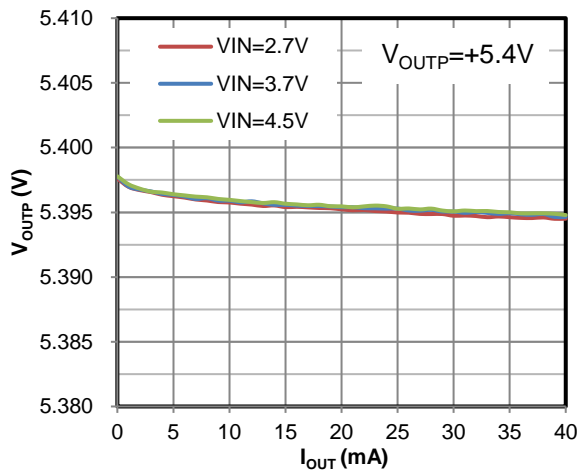
Figure 29 Load Regulation (40mA Mode)
