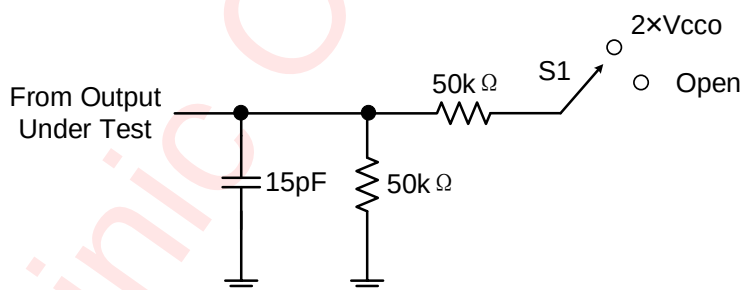
Figure 6 Load Circuit of Open-Drain Driver
