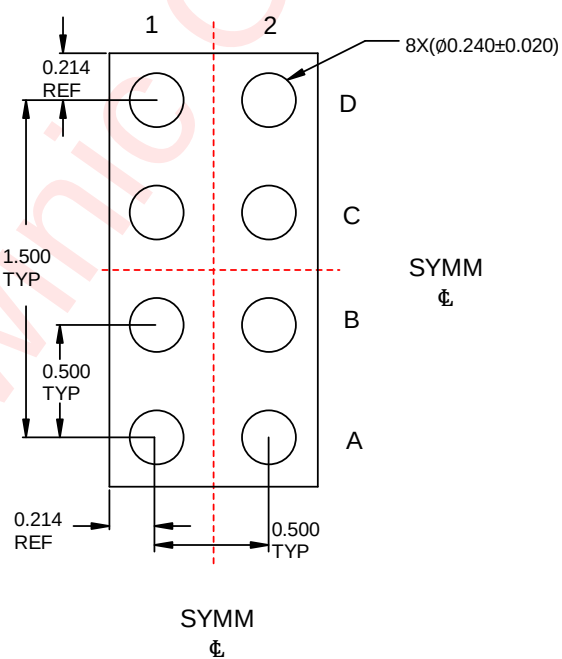
Bottom View
