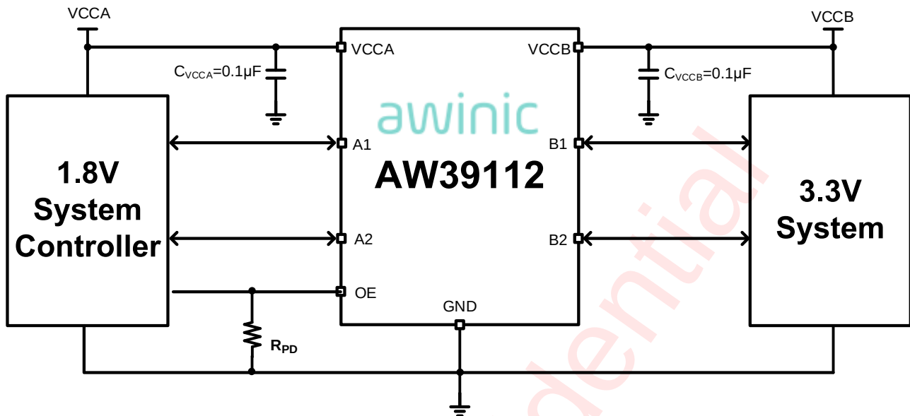
Figure 14 AW39112 Application Circuit
