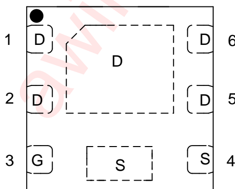
AW403002NDNR (Top View)
