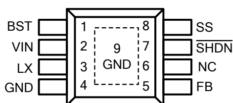
Figure 1. Pin Assignment of FR9608
