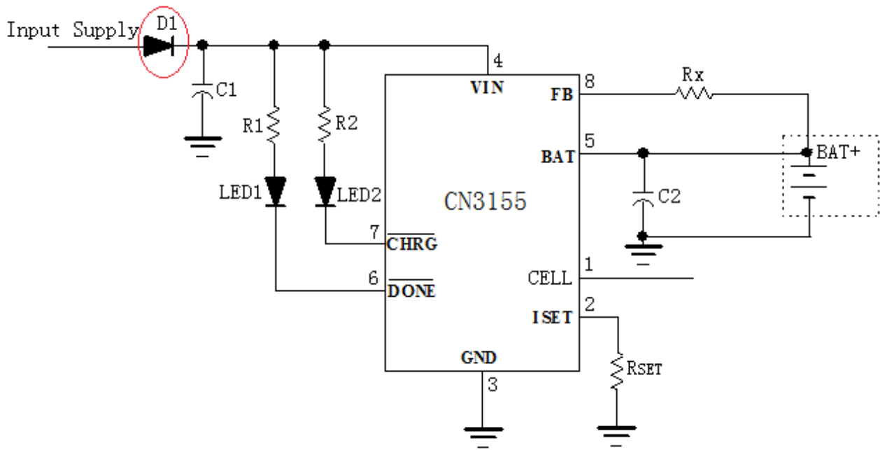
Figure 5 Adding Diode D1 to Suppress Voltage Spike
