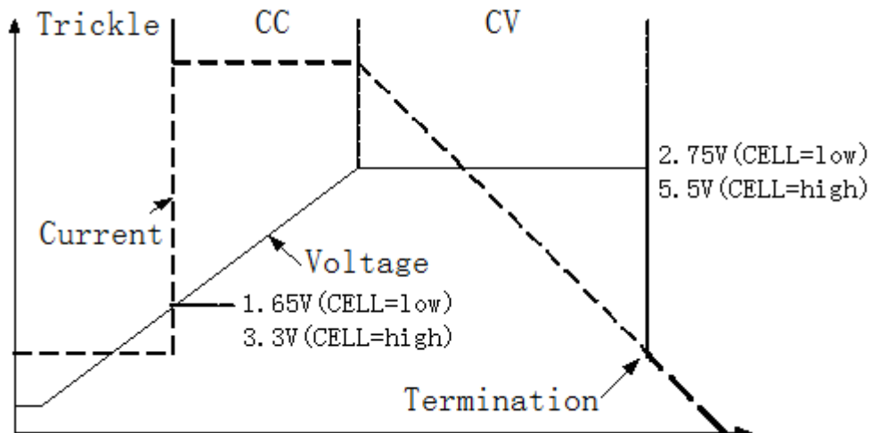
Figure 3 Charging Profile
