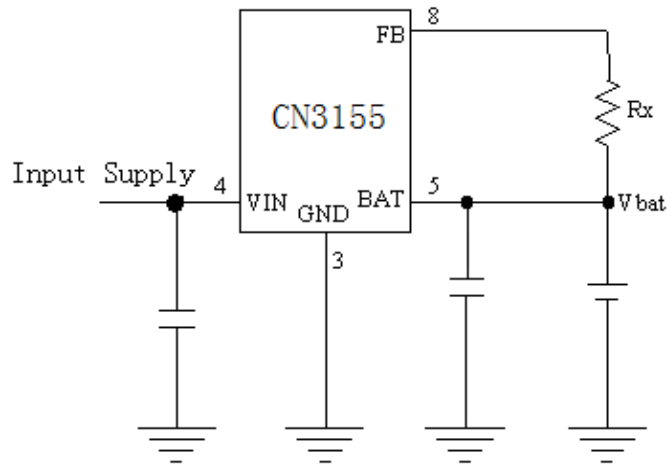
Figure 4 Adjust Regulation Voltage in Constant Voltage Mode
