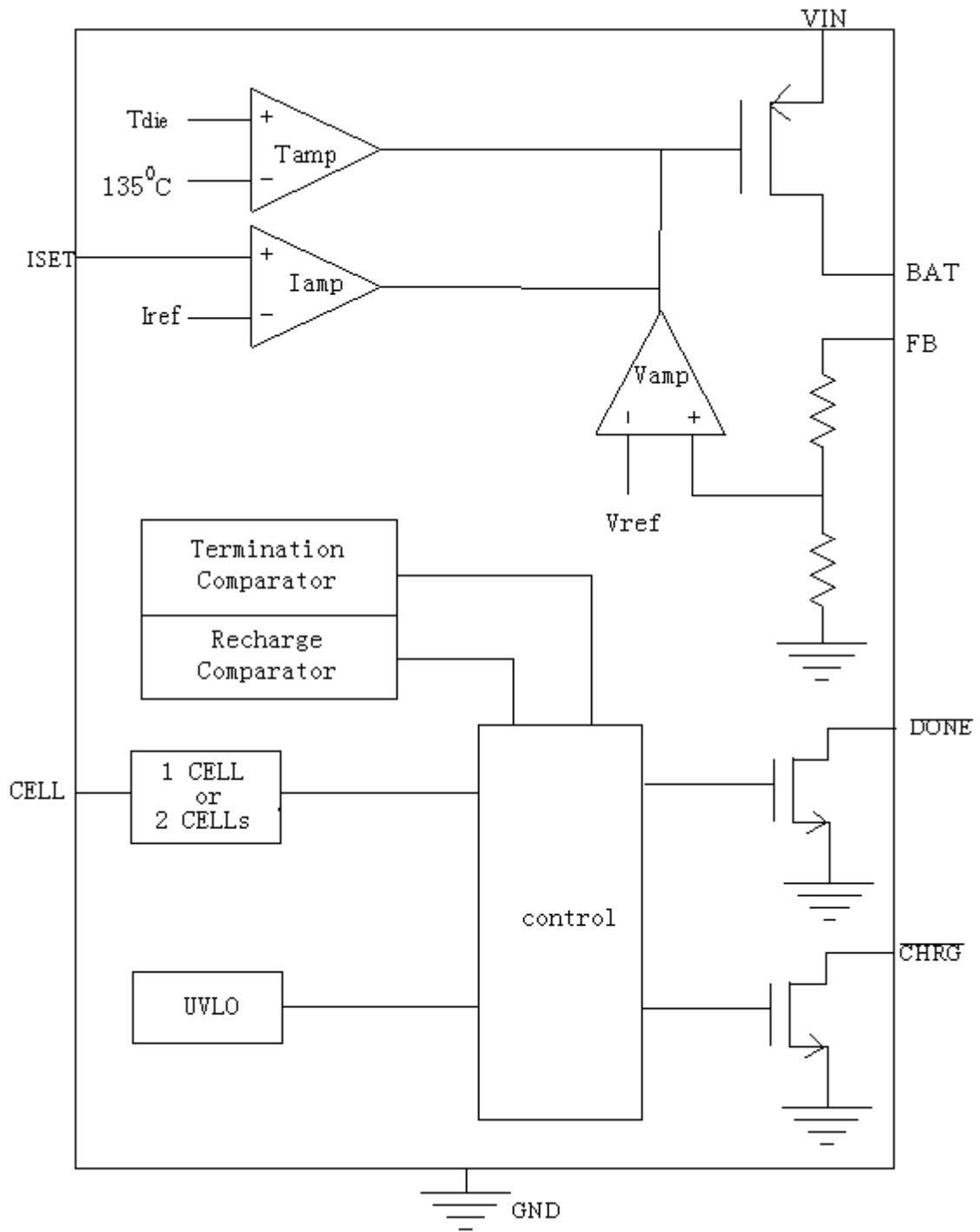
Figure 2 Block Diagram
