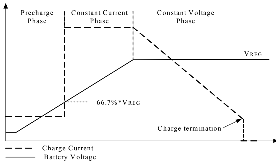
Figure 2 The Charging Profile
