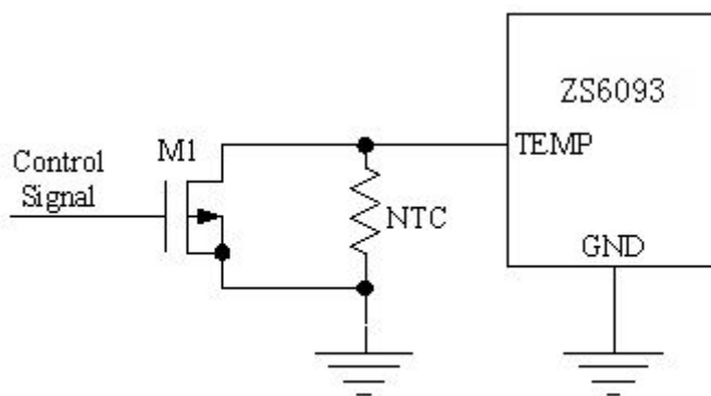
Note: M1 is N-Channel MOSFET
