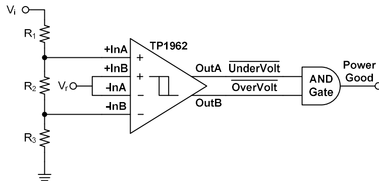
Figure 9. Windowed Comparator
