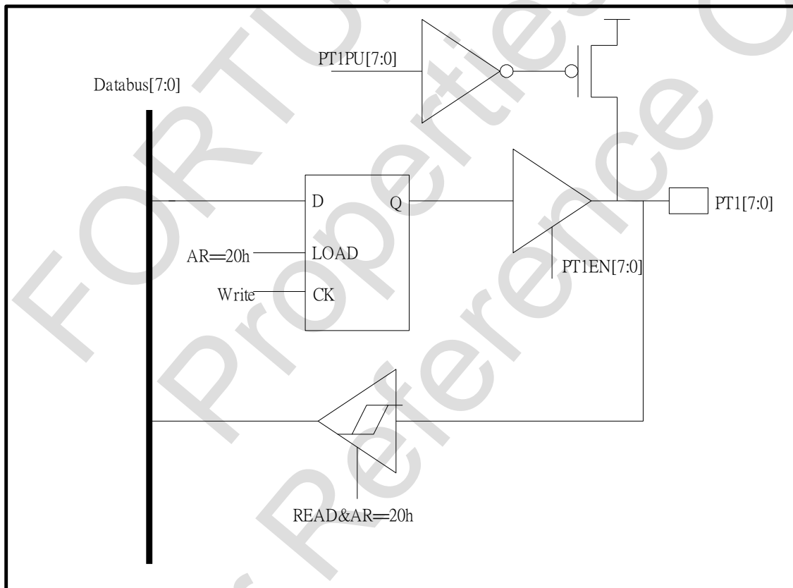
Figure 7-1 FS98024 GPIO port 1 functional block
