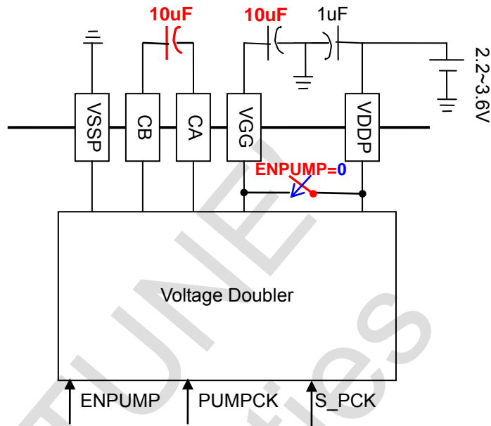
Figure 4-2 Voltage Doubler
