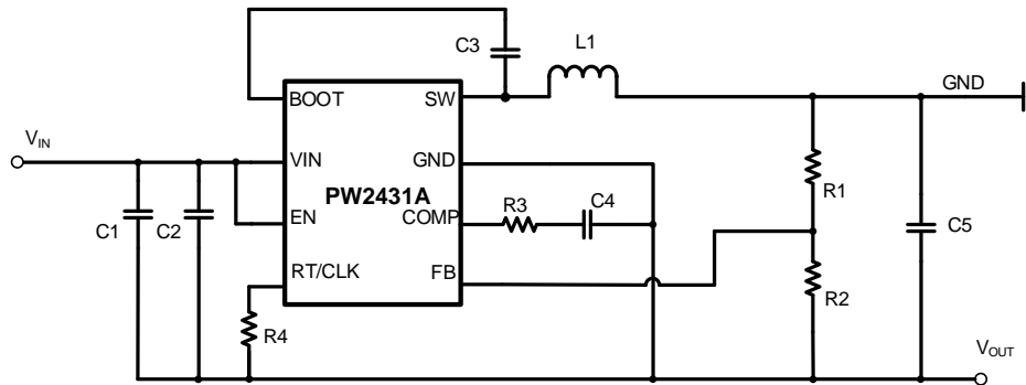
Figure 20. PW2431A Inverting Power Supply
