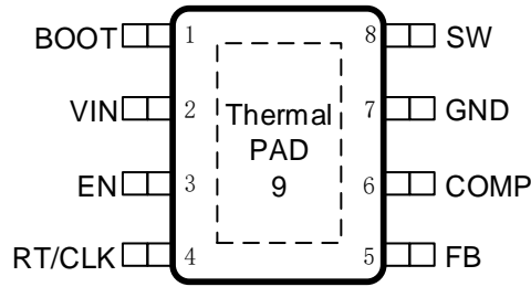
Figure 2. 8-Lead Plastic E-SOP
