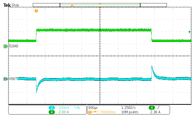
Figure 24. Load Transient (0.875A-2.625A, 250µmV/us)
