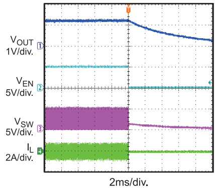
Enable Shutdown I_{OUT} = 0A , PWM
