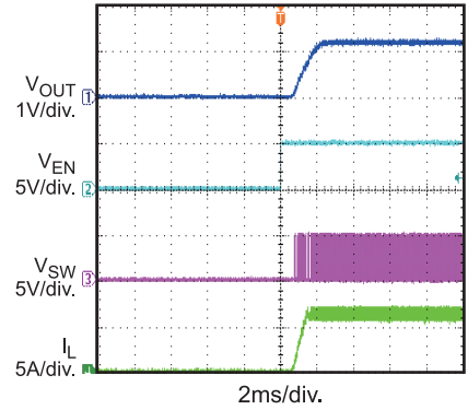
Enable On I_{OUT} = 6A , PWM
