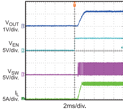
Enable On I_{OUT} = 6A , PFM
