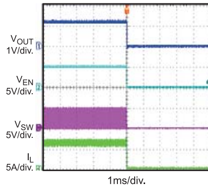
Enable Shutdown I_{OUT} = 6A , PWM
