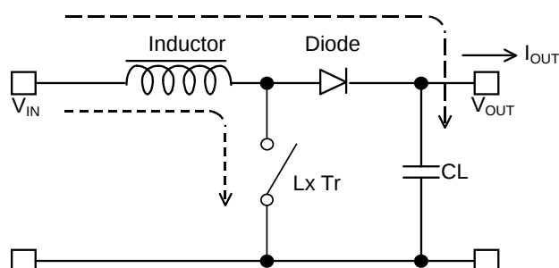
&lt;Basic Circuit&gt;
