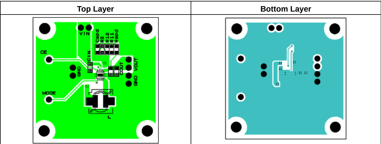
RP402K00xx (PKG: DFN(PLP)2020-8pin) Typical Board Layout
