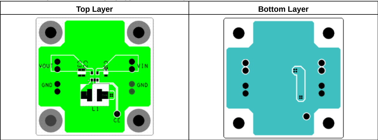
RP402Nxxxx (PKG: SOT-23-5pin) Typical Board Layout
