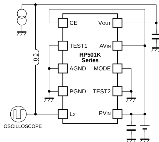
Oscillator Frequency
