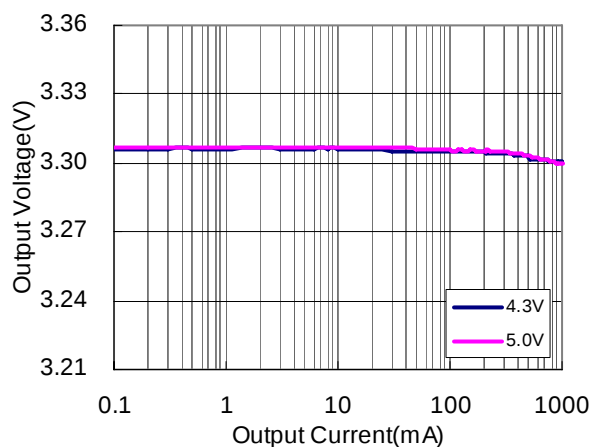
RP501K331x(PWM fixed)
