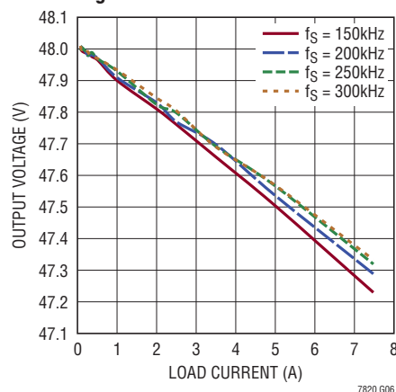
Output Voltage vs Load Current 24V to 48V Voltage Doubler in Figure 8
