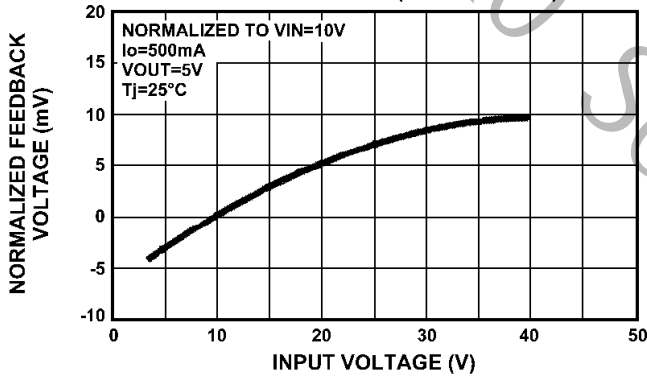
LINE REGULATION (ADJ. VERSION)
