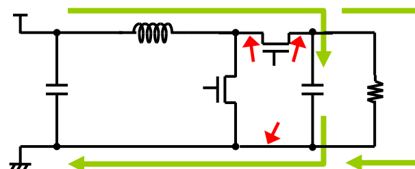
Figure 2. MOSFET-OFF
