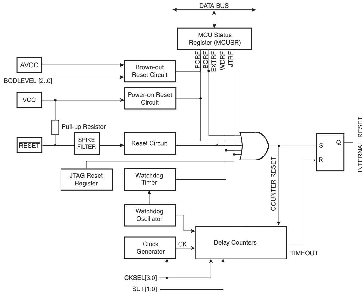
Figure 12-1. Reset Logic
