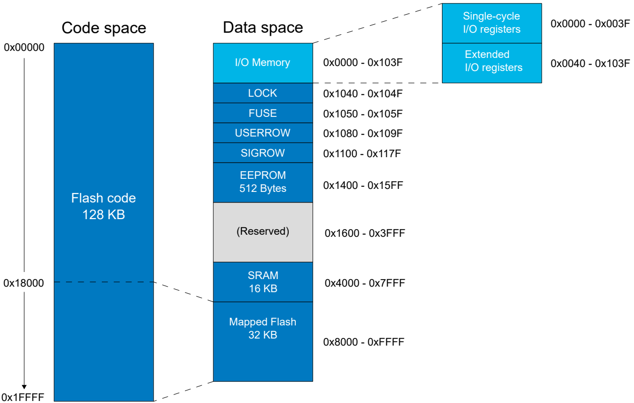
Figure 8-1. Memory Map
