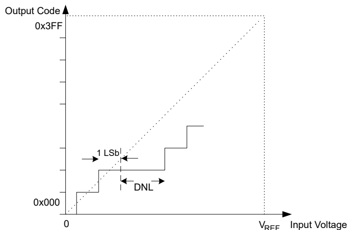
Figure 6-4. Differential Nonlinearity
