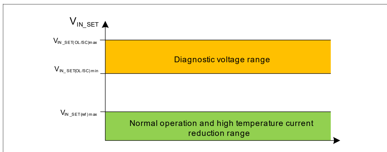
Figure 11 Voltage domains for I_{IN\_SET} pin, if ST pin is connected to GND
