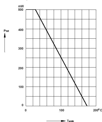
Admissible power dissipation versus ambient temperature
