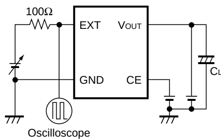
Test Circuit 4
