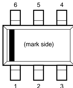
R1225N (SOT-23-6W) Pin Configuration
