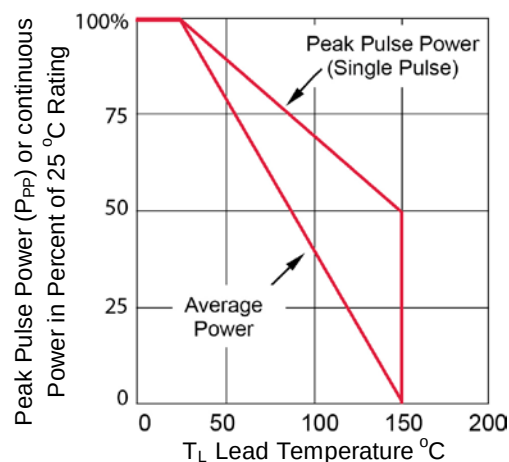
FIGURE 3 Derating Curve
