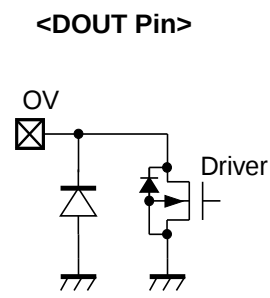
Equivalent Circuit for DOUT Pin
