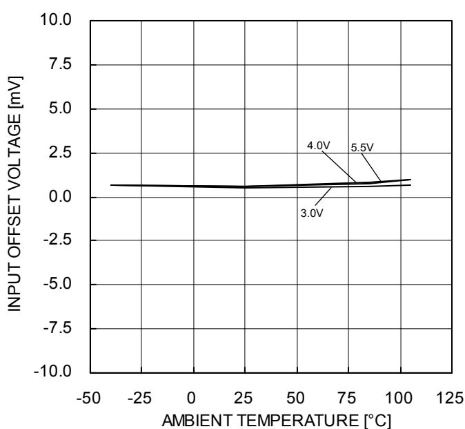
Figure 38. Input Offset Voltage vs Ambient Temperature
