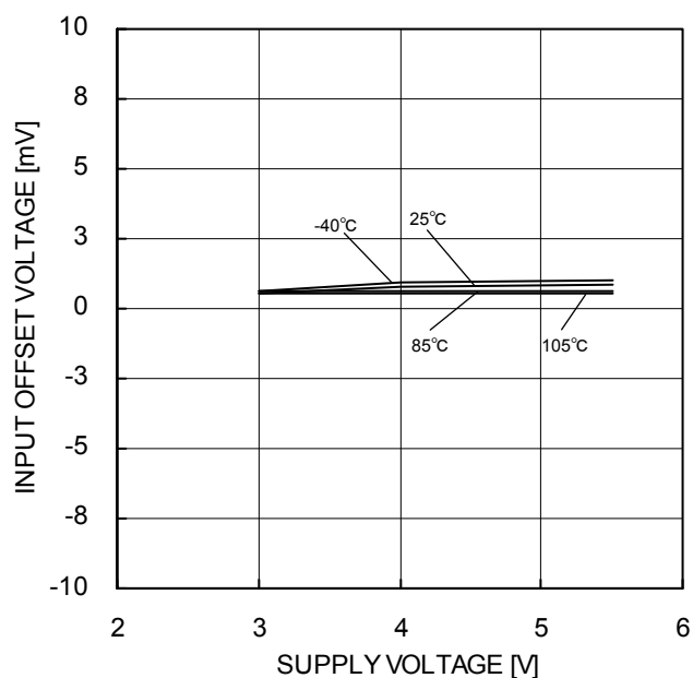
Figure 37. Input Offset Voltage vs Supply Voltage
