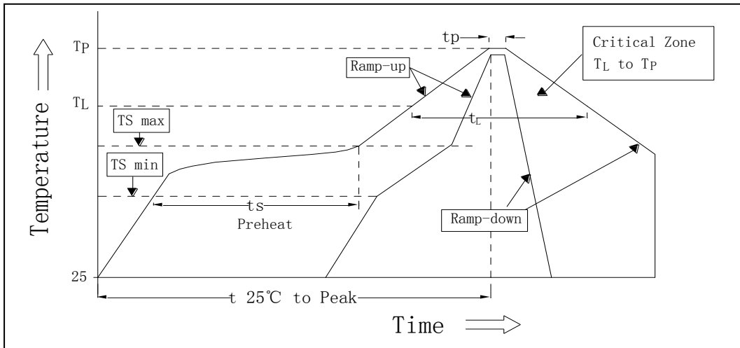
Fig.3-1 SMT Reflow Soldering Instructions SMT 回流焊说明名
