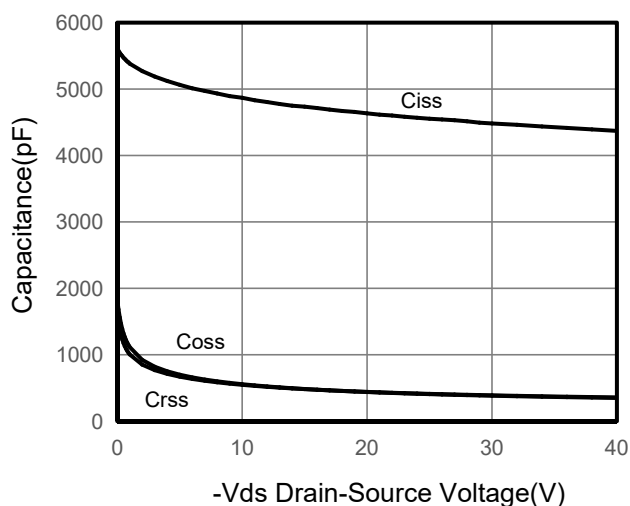
Figure 5. Capacitance
