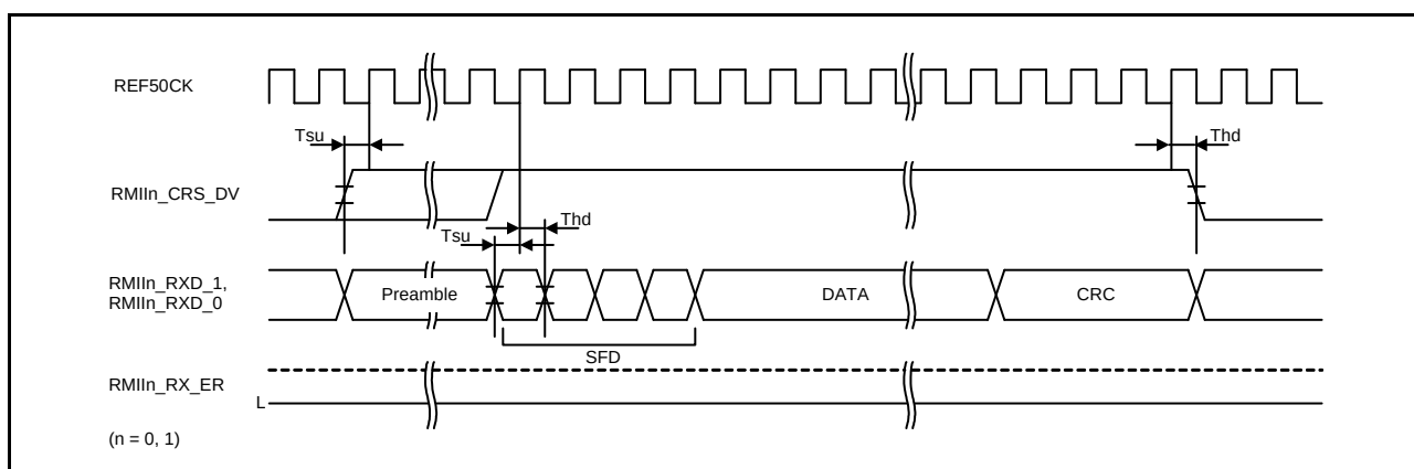
Figure 2.83 RMI Reception Timing (Normal Operation)
