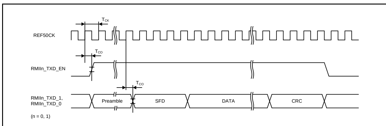
Figure 2.82 RMI Transmission Timing
