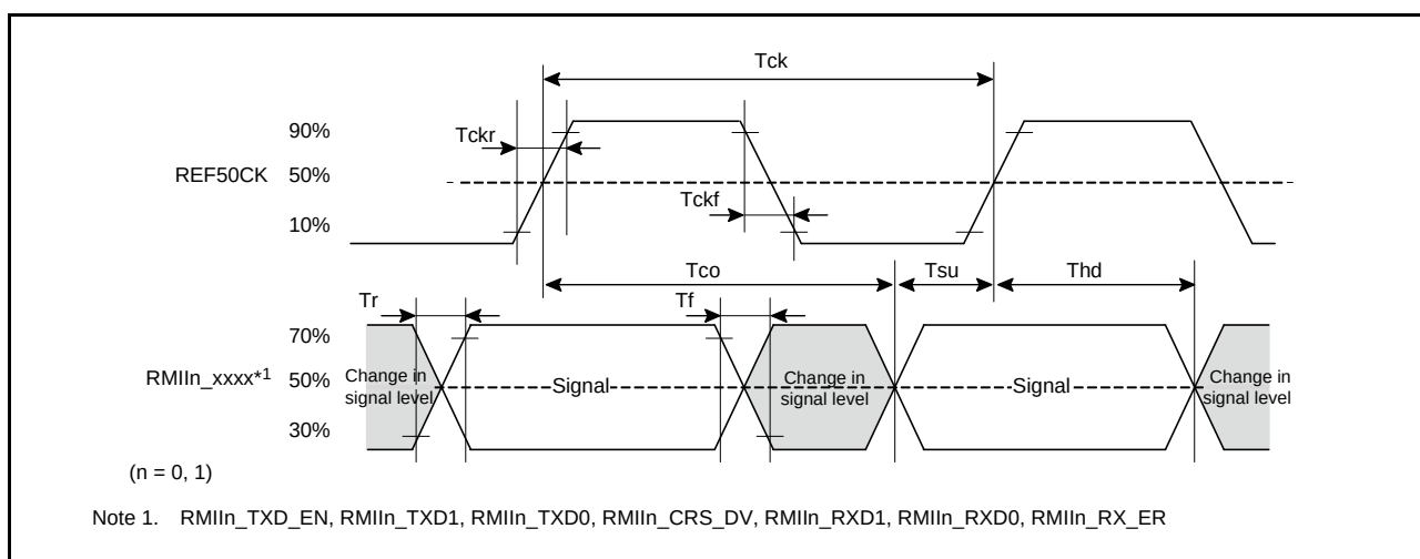
Figure 2.81 Timing with the REF50CK and RMI Signals
