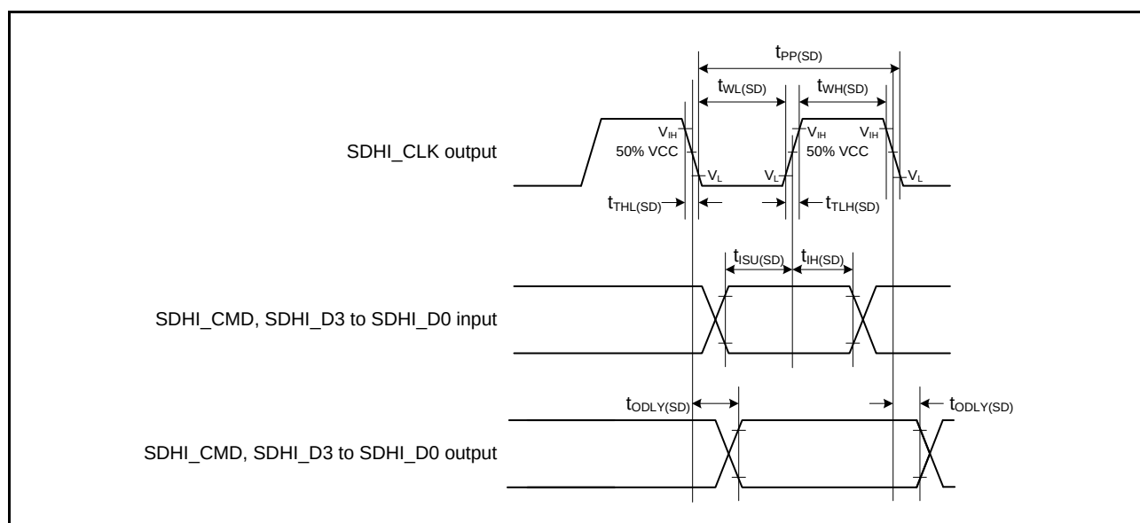
Figure 2.80 SD Host Interface Input/Output Signal Timing
