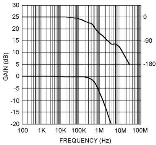
Gain / Phase Response, A_V = 2 V_{DD} = 5V , 8\Omega Load, C_{LOAD} = 500pF
