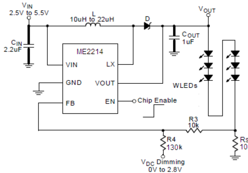
Figure 2. Dimming Control Using a DC Voltage for the ME2214
