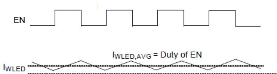
Figure 1. PWM Dimming
