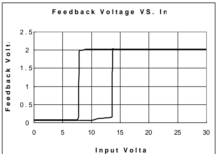
(6) Feedback Voltage VS. Input Voltage
