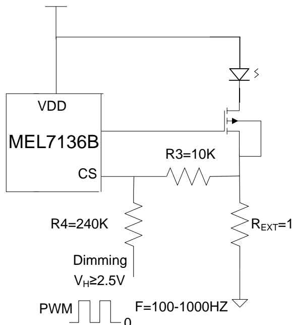
Figure 2. Dimming Control Using a PWM Signal
