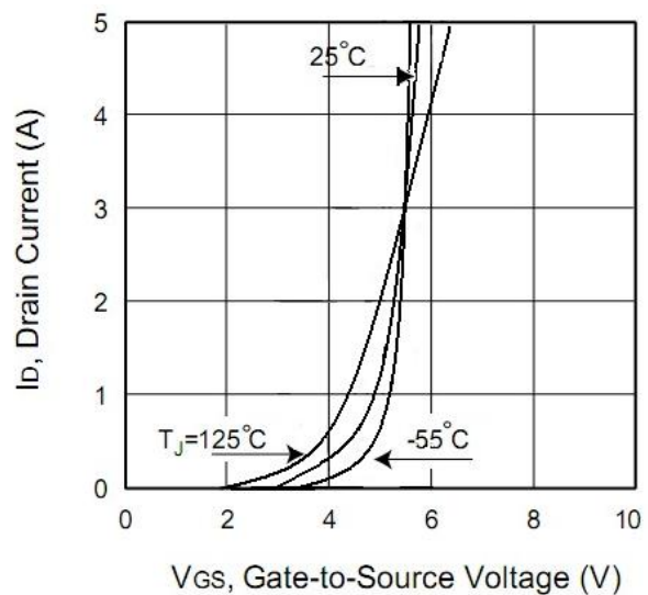
Figure 8. Transfer Characteristics
