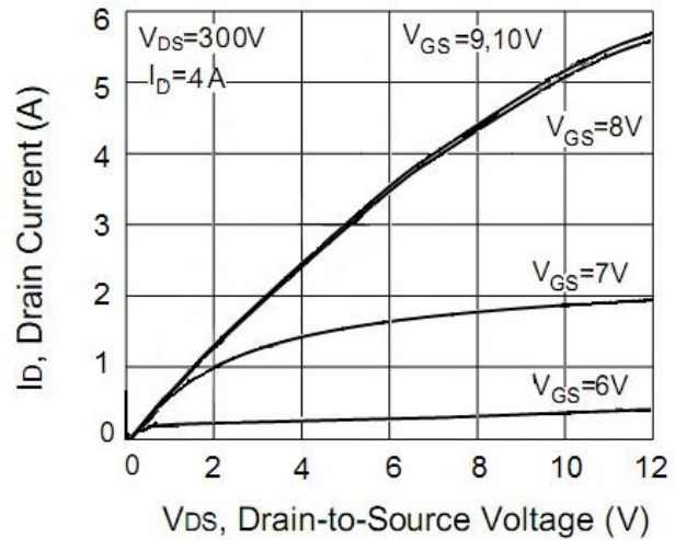
Figure 6. On-State Characteristics
