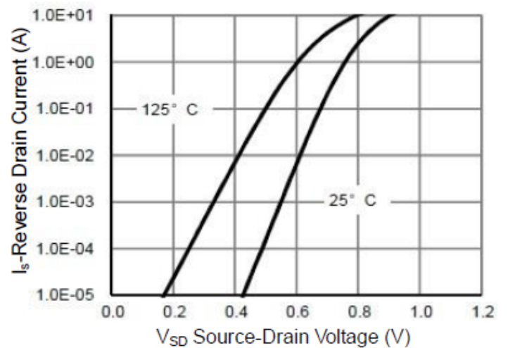
Figure6. Body-Diode Characteristics
