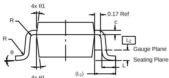
6-LEAD TSOP
