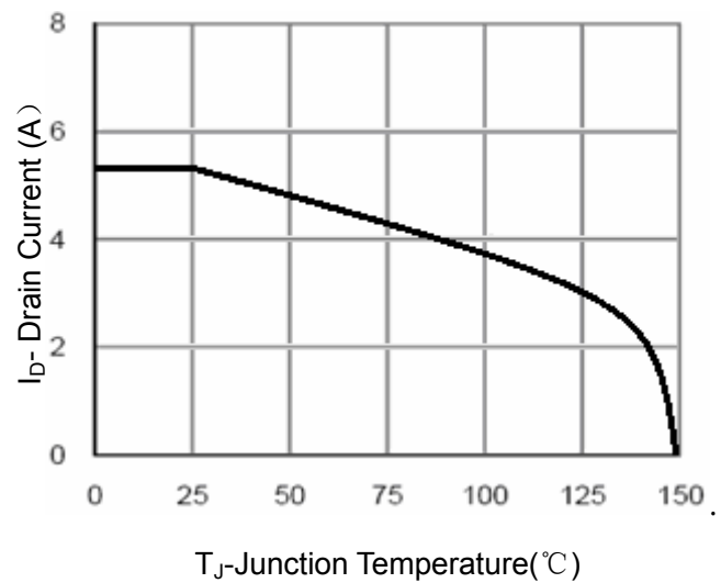
Figure 4 Drain Current
